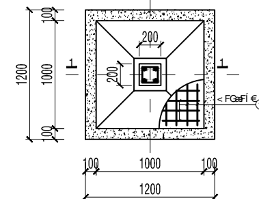
MÓNG M1, TL 1/50
